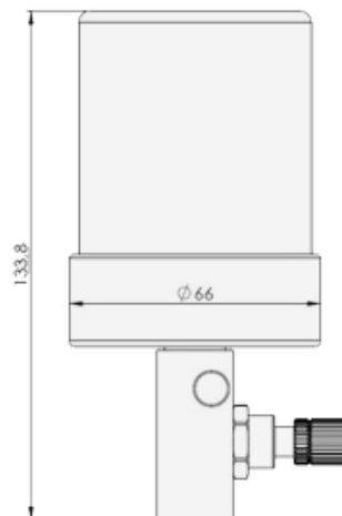
Grease version
