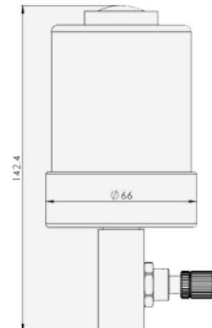
Oil version
